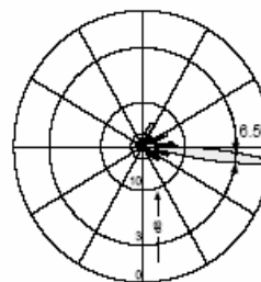
Vertical Pattern 6° electrical downtilt
