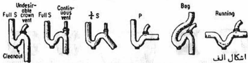
Lead traps. All styles are available, with and without cleanouts and vents
